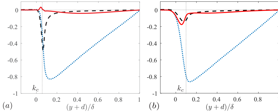
FIGURE 16. Shear stresses for cases with (a) regular and (b) random interfaces: --- Reynolds shear stress, --- viscous shear stress and — form-induced shear stress.
