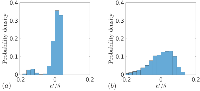
FIGURE 5. Probability density function of bed height fluctuations for the (a) regular and (b) random interfaces.
