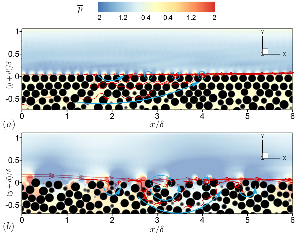
FIGURE 24. Time-averaged pressure variation and 3D mean streamlines for (a) regular and (b) random interfaces. Blue arrows indicate examples of hyporheic flow paths.
