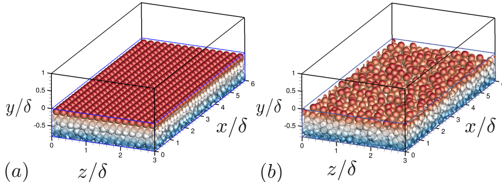
FIGURE 2. Synthesized sediment beds colored by y/\delta with (a) the regular and (b) the random interfaces.
