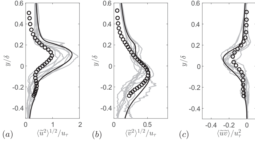
FIGURE 7. Comparison of (a) streamwise, (b) wall-normal and (c) shear component of the form-induced stress tensor. \circ Experiment, \text{—} DNS. Black lines represent the values spatially averaged over the entire horizontal plane; grey lines emulate the sampling used in the experiment.
