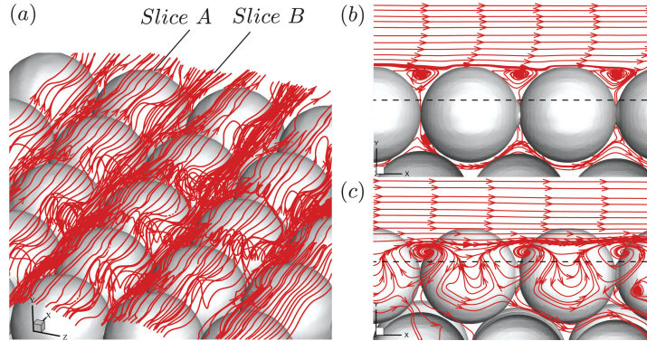
FIGURE 14. (a) Time-averaged streamlines for the regular interface. (b) Streamlines on Slice A ( x - y plane across the crests of the grains). (c) Streamlines distribution on Slice B ( x - y plane across the valley between two rows of grains). Dash lines indicate y = -d .
