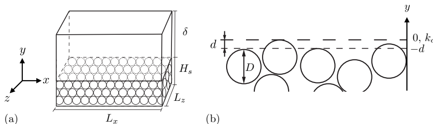
FIGURE 1. (a) Simulation domain and (b) positions of sediment crest, k_c , and zero-plane displacement, d , defined in Section 3.2.1.
