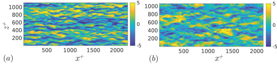
FIGURE 11. Contours of instantaneous u'^+ in the (x, z) plane at the respective \langle \overline{u'^2} \rangle -peak elevations for the (a) regular and (b) random interfaces.
