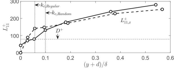
FIGURE 12. Integral length scales of u' motions along the streamwise directions for regular (---) and random (—) interfaces.
