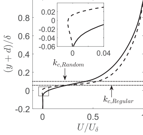
FIGURE 9. DA velocity along y in linear scaling for regular (---) and random (—) interfaces. Inset magnifies the distribution at y \approx -d .
