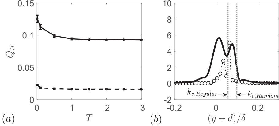
FIGURE 23. (a) Wall-normal flux at y = -d normalized by u_\tau \delta^2 with different averaging window sizes T u_\tau / \delta for regular (---) and random (—) interfaces. (b) Pressure-work term of \langle \tilde{v}^2 \rangle_s budget normalized by u_\tau^3 / \delta for regular(---, \circ ) and random(—) interfaces.
