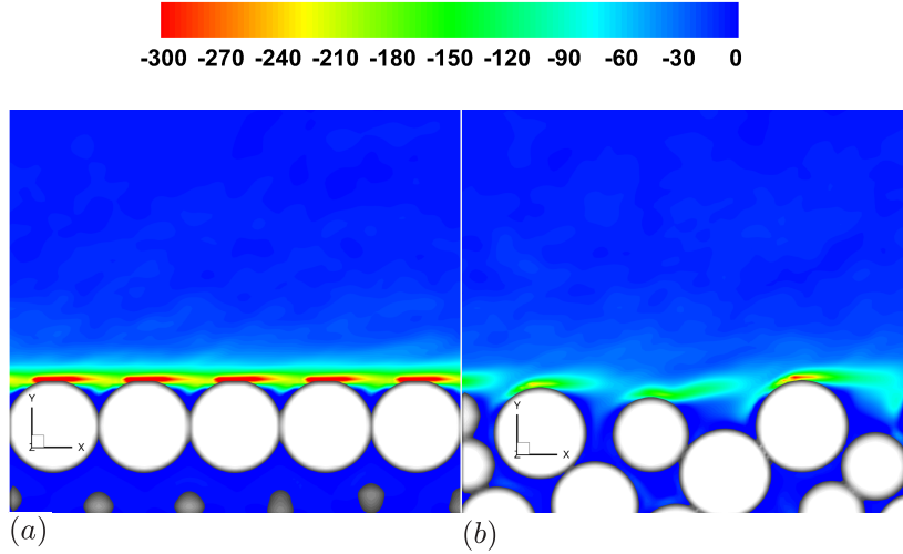
FIGURE 19. Time-averaged spanwise vorticity \bar{\omega}_z normalized by u_\tau/\delta at (a) Slice B of the regular interface and (b) Slice D of the random interface.
