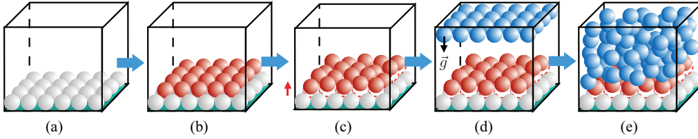
FIGURE 26. Bed synthesis with regular interface packing.
