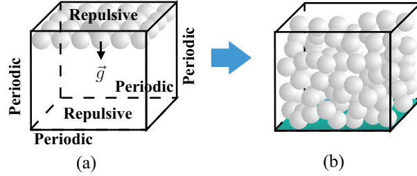
FIGURE 25. Bed synthesis with random interface packing.
