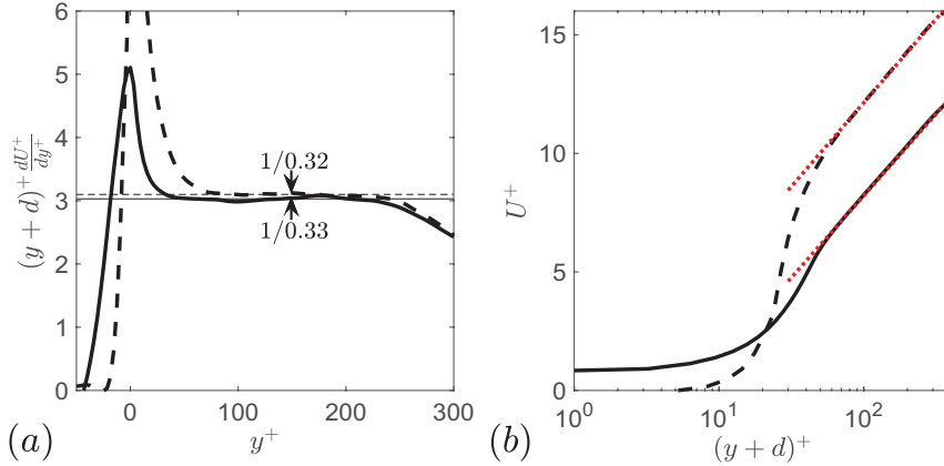
FIGURE 8. (a) Diagnostic function for fitting the logarithmic profile and (b) DA velocity profiles for regular (---) and random (—) interfaces; -.-.- fitted logarithmic profiles.
