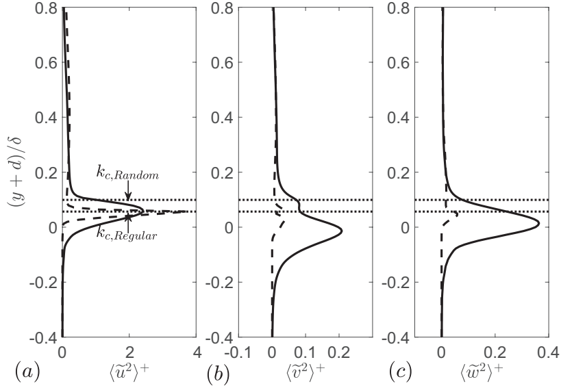
FIGURE 13. Components of the form-induced stress tensor: (a) streamwise, (b) wall-normal and (c) spanwise components, for regular (---) and random (—) interfaces.
