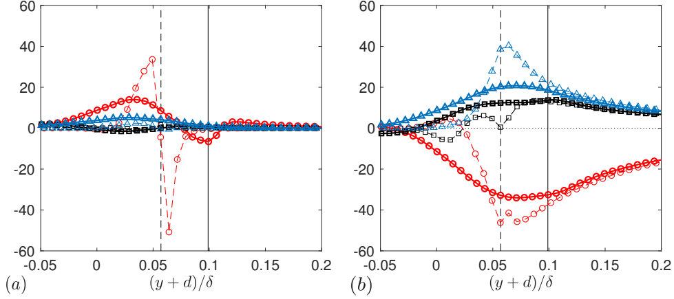
FIGURE 18. (a) Form-induced production and (b) pressure-strain-rate term in regular (---) and random interface (—) cases for the budgets of \langle u'^2 \rangle_s ( \circ ), \langle v'^2 \rangle_s ( \square ) and \langle w'^2 \rangle_s ( \triangle ); normalization is done with u_\tau and \delta .
