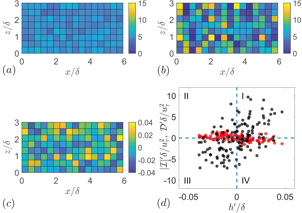
FIGURE 22. Horizontal variation of local volume-averaged \mathcal{D} (a) and |\mathcal{I}| (b), both normalized by u_\tau^2/\delta . (c) sediment surface height fluctuations h' normalized by \delta for the random-interface case. (d) Correlations of \mathcal{D}' (red) and |\mathcal{I}'| (black) with h' .
