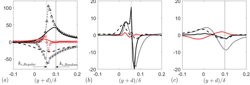
FIGURE 17. Terms in the TKE budget equation. (a) Production and viscous dissipation for regular (symbols and thin lines) and random-interface (thick lines) cases; P_s (—, \Delta ), P_m + P_w (—, \circ ) and \epsilon (---, \square ). Transport terms for (b) regular and (c) random interfaces; T_w (—), T_t (---), T_\nu (—) and T_p (---). All terms are normalized by u_\tau^3/\delta .
