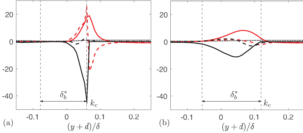
FIGURE 21. Terms in the DA u -momentum equation (equation (3.9)), normalized by u_\tau^2/\delta for (a) regular and (b) random interfaces: Reynolds-stress term (—), viscous stress term (---), total drag (——), form-induced stress term (---) and pressure-gradient term(···).
