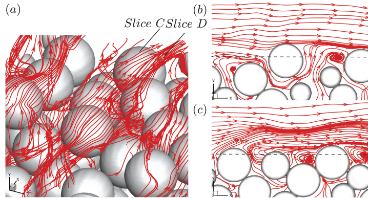
FIGURE 15. (a) Time-averaged streamlines for the random interface. (b) and (c) show streamlines on two x - y planes, Slice C and Slice D. Dash lines indicate y = -d .
