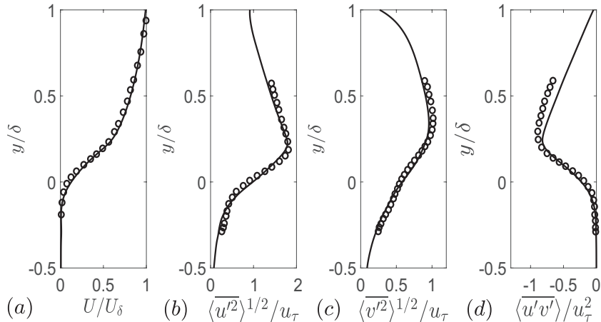
FIGURE 6. Comparison of (a) mean velocity and (b-d) streamwise, wall-normal and shear components of the Reynolds stress tensor. \circ Experiment, \text{—} DNS.
