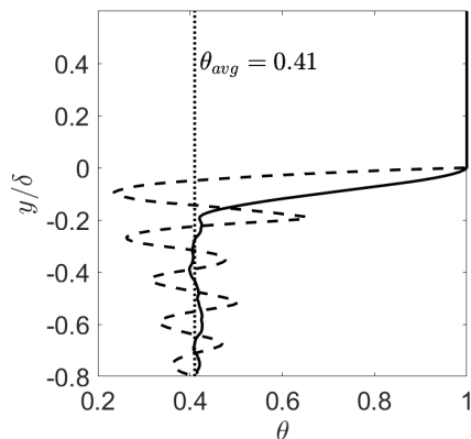
FIGURE 3. Wall-normal profiles of plane-averaged porosity profile for regular (---) and random (—) interfaces.
