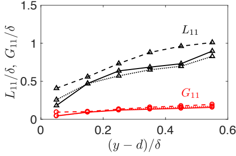
Figure 5. Integral length scale of u' motions in the outer layer.
