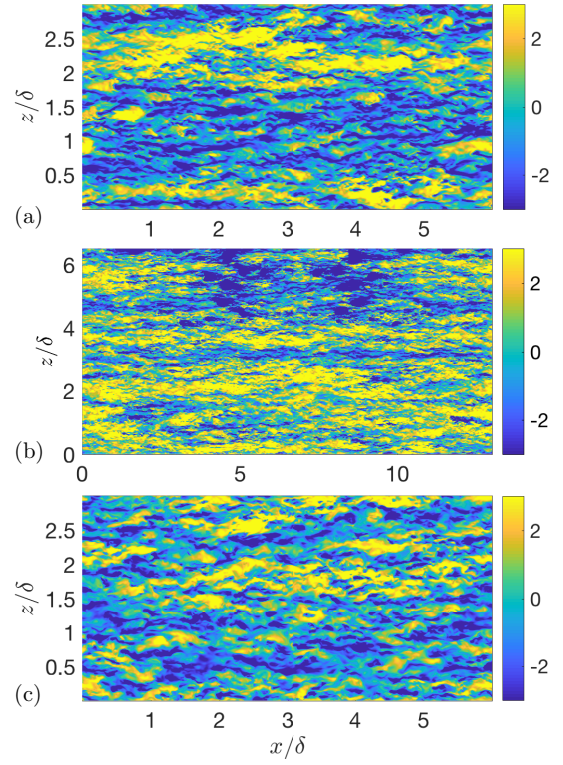
Figure 6. Contours of instantaneous u'^+ at (y-d)/\delta = 0.05 for (a) SM, (b) TB (one half is shown), (c) SG.
