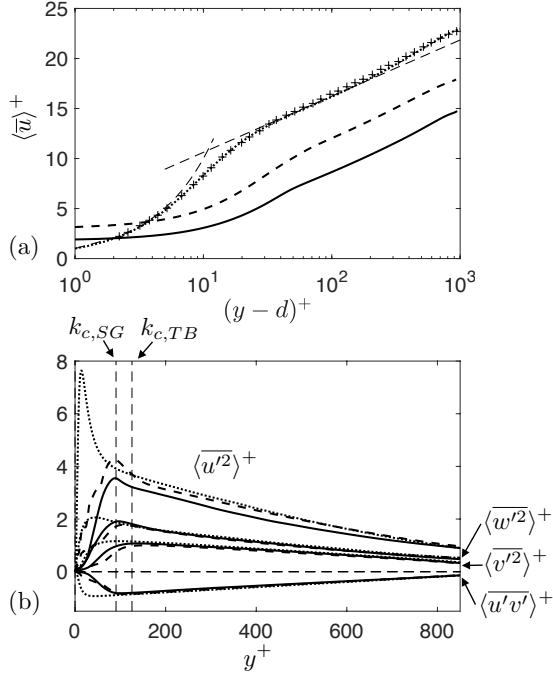
Figure 2. (a) Double-averaged velocity and (b) Reynolds stresses. + smooth-wall experiments (Schultz & Flack, 2013).
