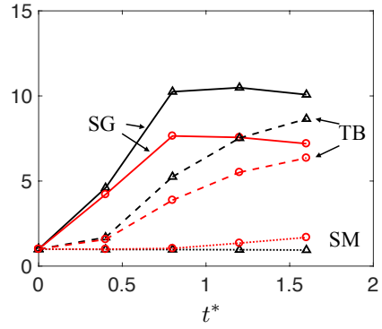
Figure 9. Variables of peak values of Reynolds shear stresses (black \triangle ) and TKE (red \circ ) in transient channels, normalized by u_\tau^2 of the initial developed channel.
