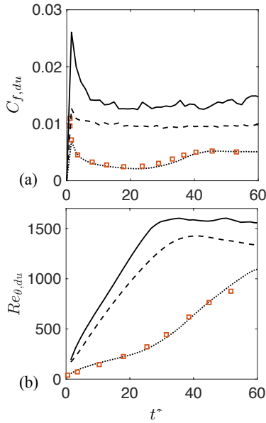
Figure 8. Boundary layer parameters of the differential flow in transient channels: (a) friction coefficient and (b) Reynolds number. \square DNS by He & Seddighi (2013).
