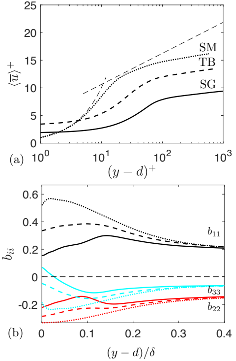
Figure 10. (a) Mean velocity and (b) Reynolds-stress anisotropy for all transient cases at t^* = 0.4 .
