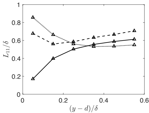
Figure 11. Integral length scale for all transient cases at t^* = 0.4 .
