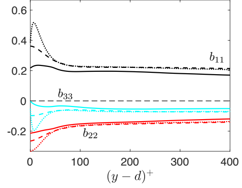
Figure 3. Reynolds stress anisotropy for all cases
