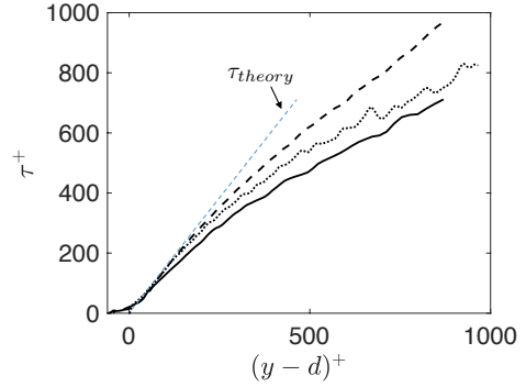
Figure 7. Comparison of turbulent time scale.
