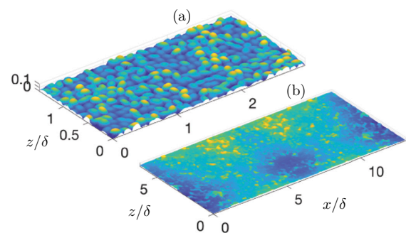
Figure 1. Surfaces colored by height. (a) one quarter of SG surface (zoomed in). (b) one half of TB surface.
