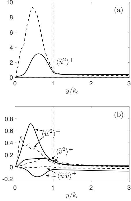
Figure 4. Double-averaged dispersive stresses.
