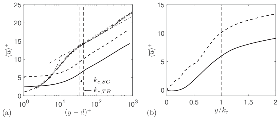
FIG. 3. DA velocity against (a) logarithmic and (b) linear y coordinates. --- SM, — SG, and - - - TB. + Smooth-wall experiment [37]. Thin dashed lines indicate crest locations.
