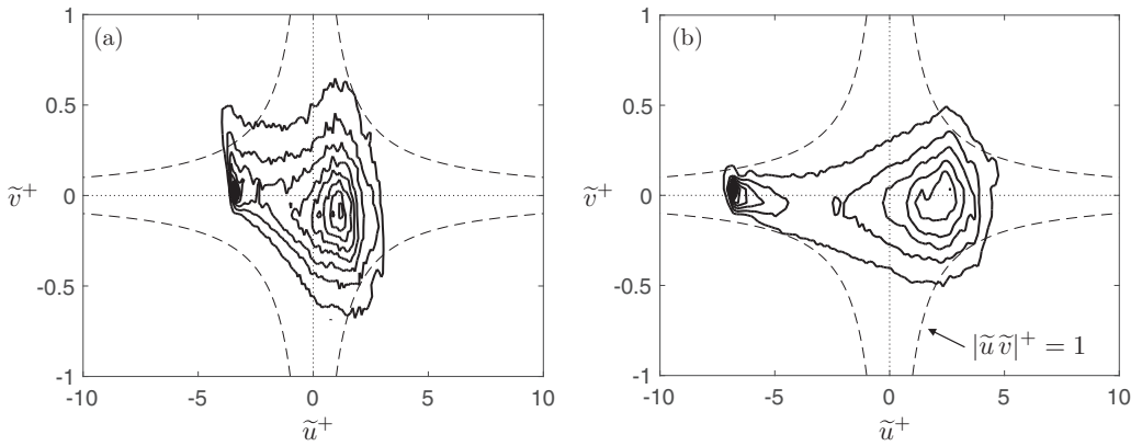
FIG. 8. Joint probability density function of \tilde{u} and \tilde{v} for (a) SG and (b) TB at y/d = 1 . Contour line values (in wall units) range from 0.05 to 0.5 with step size 0.05.
