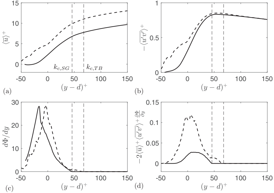
FIG. 14. [(a)–(c)] Contributing factors to (d) P_m for the rough cases. — SG, --- TB.
