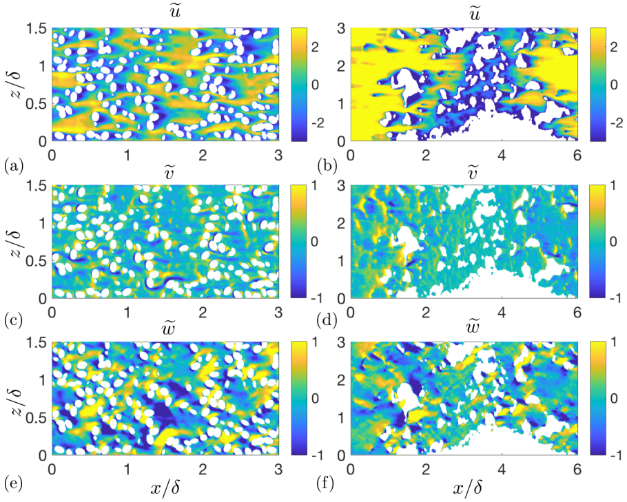
FIG. 7. Form-induced fluctuations in plus units for SG [(a), (c), (e)] and TB [(b), (d), (f)] in the wall-parallel plane at y/d = 1 . White region is within solid.
