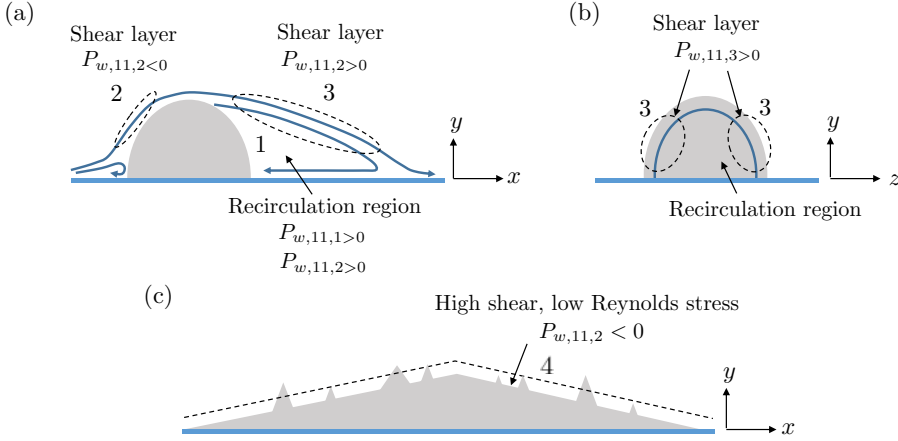
FIG. 16. Sketches of local flow characteristics to explain P_{w,11} distribution in Figs. 15(a) and 15(d): Typical flows around an isolated protuberance in (a) (x, y) plane and (b) (y, z) plane (viewed towards +x direction, and (c) over a large-wavelength surface undulation. Numbers 1–4 indicate flow characteristics discussed in text.
