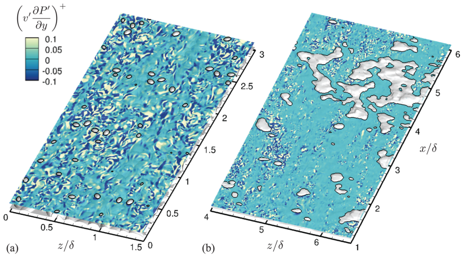
FIG. 12. Instantaneous rate of work of pressure fluctuations against wall-normal velocity fluctuations at (y - d)^+ = 25 on (a) SG and (b) TB. Roughness surfaces are shown in white.
