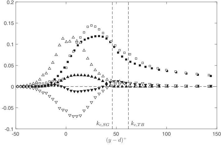
FIG. 13. Breakdown of total production of streamwise Reynolds stress for SG (filled symbols) and TB (empty symbols). Symbols: \square , P_s ; \triangle , P_m ; \nabla , P_w .
