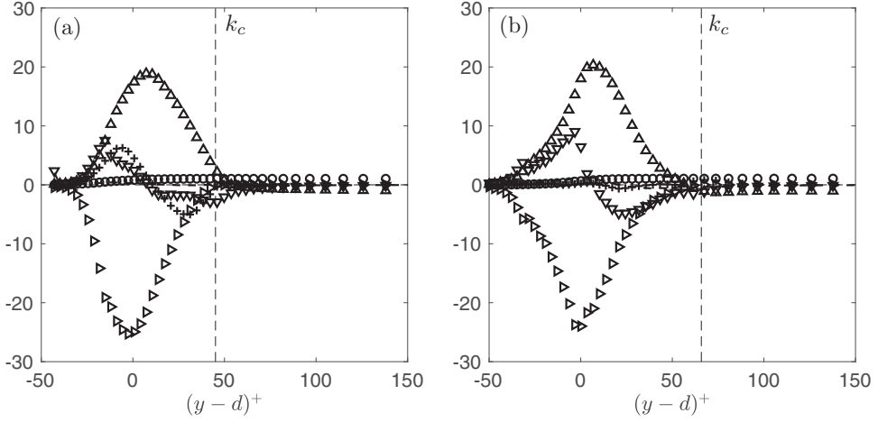
FIG. 9. Mean momentum balance for (a) SG and (b) TB, normalized in wall units. Symbols: \circ , pressure gradient; \nabla , viscous force; \triangle , turbulence inertia; + , dispersive term; \triangleright , total drag; and - - , residual.
