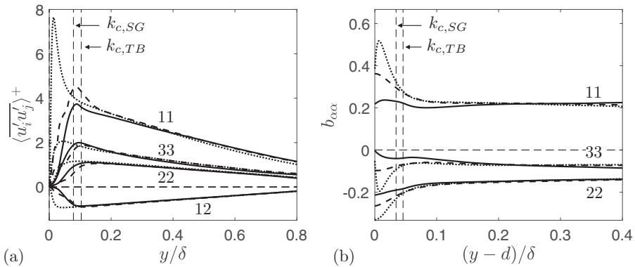
FIG. 5. Tensor components of (a) Reynolds stress and (b) its anisotropy. --- SM, — SG, - - - TB.
