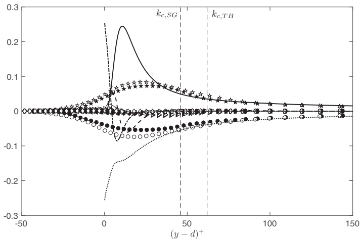
FIG. 10. TKE budget terms in wall units for SM (lines), SG (filled symbols), and TB (empty symbols). Lines: —, P_s ; ---, T_i ; ···, T_v ; — (thin), T_p ; -·-, \epsilon . Symbols: \star , (P_s + P_w + P_m) ; \triangleright , T_i ; \triangleleft , T_v ; \diamond , T_p ; \circ , \epsilon .
