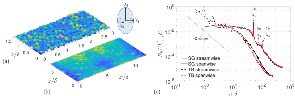
FIG. 1. Rough surfaces colored by heights of (a) one quarter of SG surface and (b) one half of TB surface. (c) Power spectra of height fluctuations with wave number \kappa_r in x and z .
