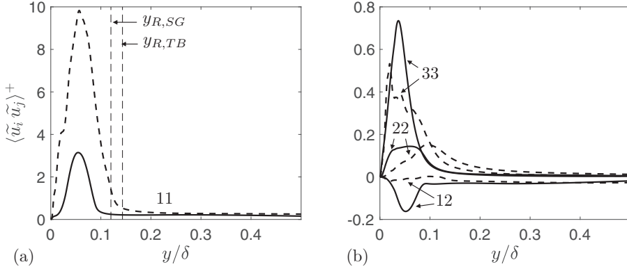
FIG. 6. Tensor components of dispersive stress.— SG; --- TB.
